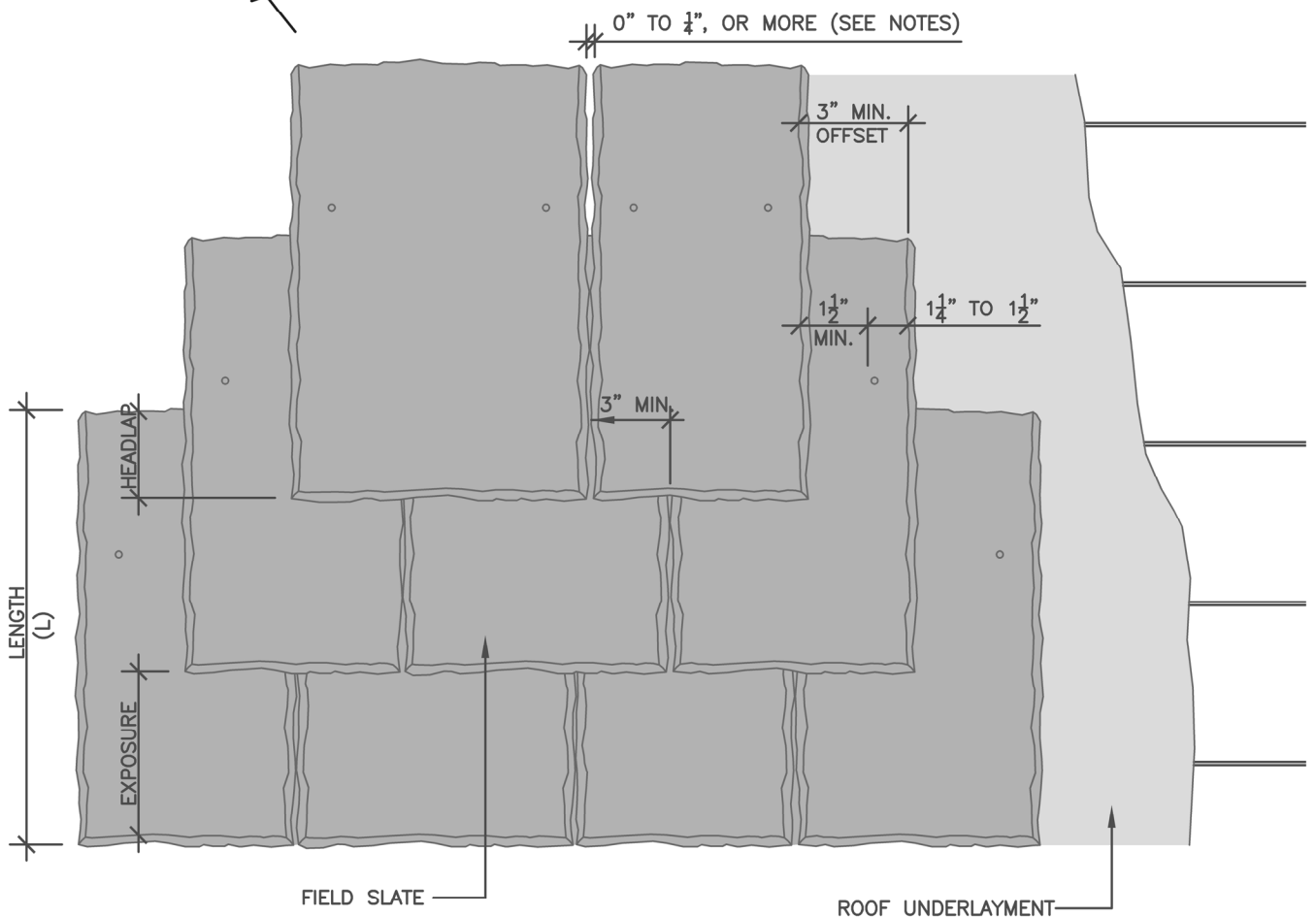
DETAIL 5-B FIELD SLATES OF RANDOM WIDTHS N.T.S.
